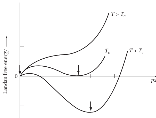
Figure 17 Landau free energy function versus (polarization) 2 in a first-order transition, at representative temperatures. At T_c the Landau function has equal minima at P = 0 and at a finite P as shown. For T below T_c the absolute minimum is at larger values of P ; as T passes through T_c there is a discontinuous change in the position of the absolute minimum. The arrows mark the minima.
