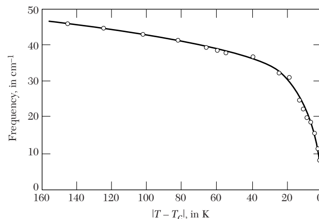
Figure 14 Decrease of a transverse phonon frequency as the Curie temperature is approached from below, in the ferroelectric crystal antimony sulphoiodide, \text{SbSI} . (After Raman scattering experiments by C. H. Perry and D. K. Agrawal.)
